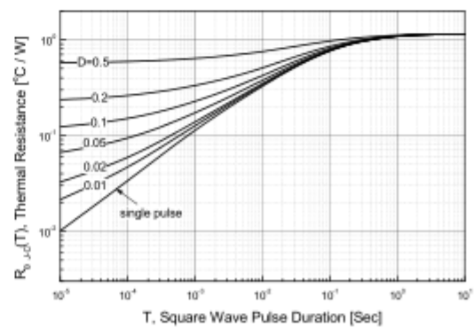
Figure 6. Transient Thermal Response Curve
