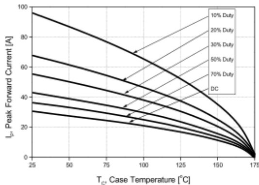
Figure 3. Derating Curve I_p - T_c
